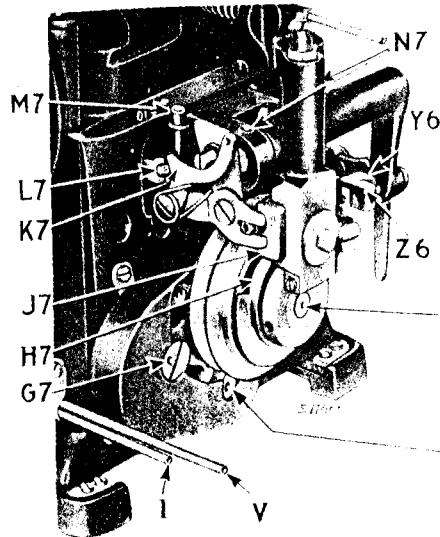
Fig. 10. View of Stop Motion Showing Shaft Speeds
